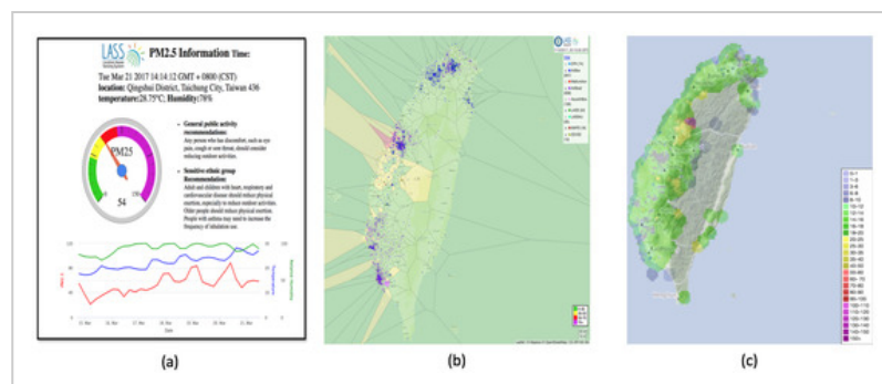
Figure 5. Data Visualization Platforms: (a) device status; (b) Voronoi diagram; and (c) real-time PM 2.5 visualization.
