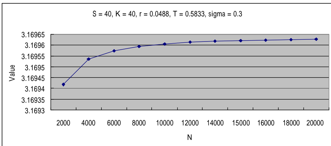
Figure A.5 the convergence of seven-month American put options
