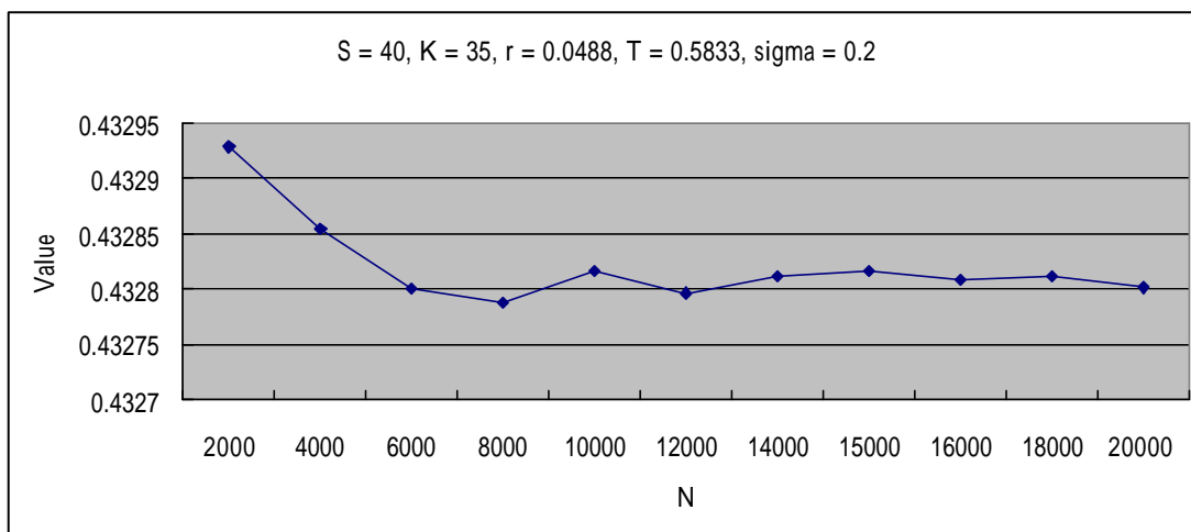
Figure A.1 the convergence of seven-month American put options
