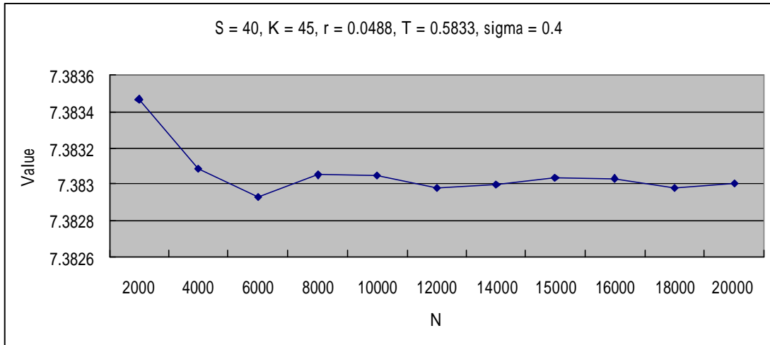
Figure A.9 the convergence of seven-month American put options
