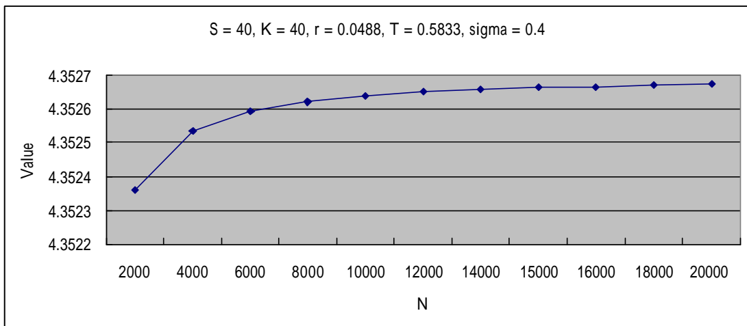
Figure A.8 the convergence of seven-month American put options
