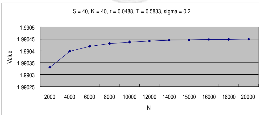
Figure A.2 the convergence of seven-month American put options
