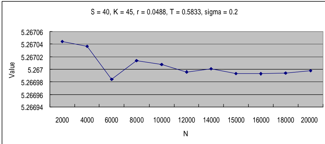
Figure A.3 the convergence of seven-month American put options
