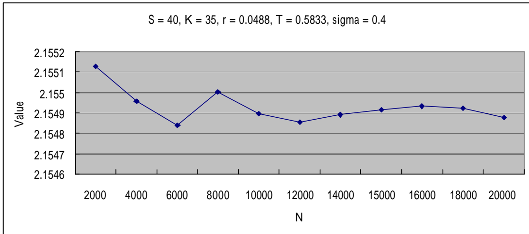
Figure A.7 the convergence of seven-month American put options
