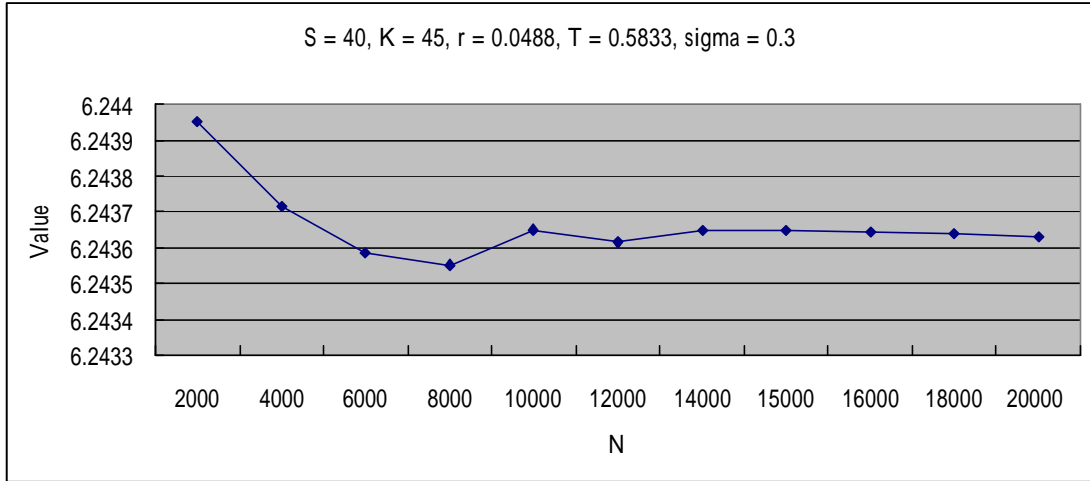
Figure A.6 the convergence of seven-month American put options
