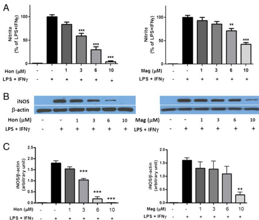
Figure 3 Hon and Mag inhibit LPS + IFN- \gamma -induced NO production and iNOS expression in BV-2 microglial cells. Cells were treated with Hon or Mag (1 to 10 \mu M) for 1 h followed by stimulation with LPS (100 ng/ml) + IFN \gamma (10 ng/ml) for 16 h. (A) Culture media were collected for determination of NO using the Griess reaction protocol as described in text. (B) Representative Western blots of iNOS protein and \beta -actin. (C) Bar graphs representing iNOS/ \beta -actin ratios. Results were expressed as the mean \pm SEM ( n = 3 ) and significant difference from the respective LPS + IFN \gamma stimulated group was determined by one-way ANOVA followed by Dunnett's tests, ** P < 0.01 ; *** P < 0.001 .
