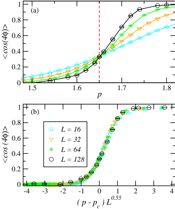
FIG. 16: (Color online) The quantity \langle \cos(4\phi) \rangle with \phi = \arctan(d_y/d_x) measures the degree of Z_4 symmetry in the VBS order parameter and also gives a good estimate of the location of the liquid-VBS transition. In the spin liquid the distribution P(d_x, d_y) is U(1) symmetric, leading to \langle \cos(4\phi) \rangle = 0 for L \rightarrow \infty , while in the columnar VBS phase, where the distribution is Z_4 -symmetric, \langle \cos(4\phi) \rangle approaches 1. (a) The curves for different system sizes cross at a single point located at p = 1.65 , which is identified as the transition point; p_{2c} = 1.650(5) . Since \langle \cos(4\phi) \rangle > 0 at this point, there is no emergent U(1) symmetry at this transition, although it appears to be a continuous transition based on other results. (b) When p - p_{2c} is scaled with the system size L raised to the power L^{1/a\nu} , with a\nu \approx 1.82 , the curves for different systems collapse onto each other.
