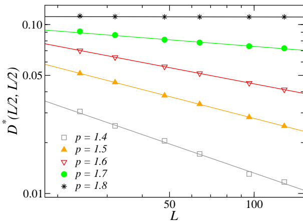
FIG. 14: (Color online) Long-distance columnar dimer correlation function versus system size for different p in the intermediate region. The correlations decay as a power-laws (with the decay exponent \beta = 0.57 for p = 1.4 , 0.43 for p = 1.5 , and 0.32 for p = 1.6 ), in the spin liquid phase and are size independent in the VBS state ( p = 1.8 ). At p = 1.7 the behavior is approximately a power-law but with a slight up-turn for the largest size, indicating a weakly VBS ordered state here.
