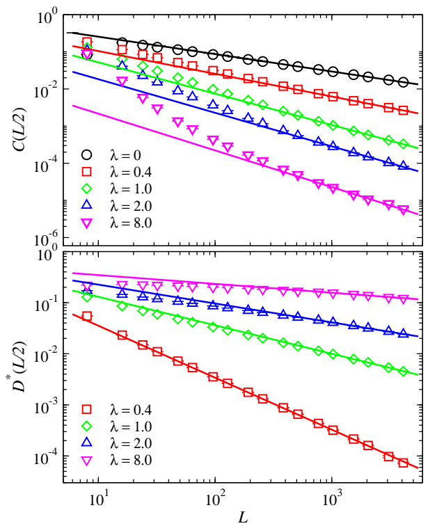
FIG. 5: (Color online) Staggered spin-spin (upper panel) and dimer-dimer (lower panel) correlations of 1D AP states at the largest distance, graphed versus the chain length at \kappa = \kappa_c for different short-bond amplitudes \lambda . All lines are fits to the form aL^{-b} .
