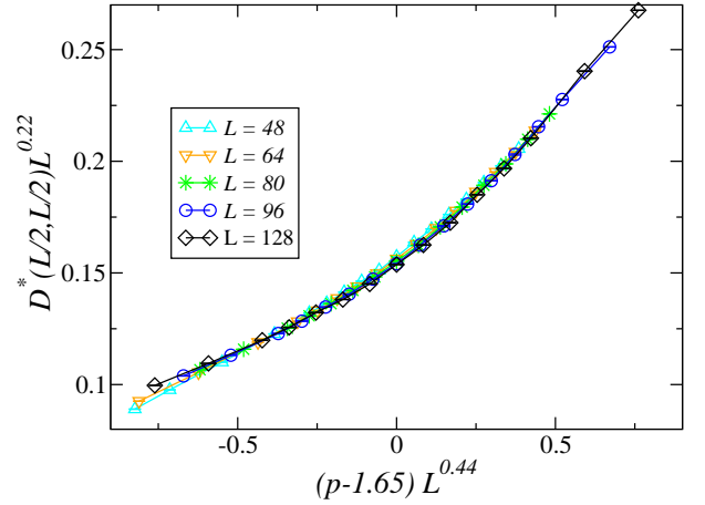
FIG. 18: (Color online) The data of Fig 11(b) in the neighborhood of the liquid-VBS transition, rescaled to extract the exponent \beta of the dimer correlation function, D^*(r) \sim r^{-\beta} , here with \beta = 0.22 , and the correlation length exponent \nu , here with \nu \approx 1/0.44 \approx 2.27 .
