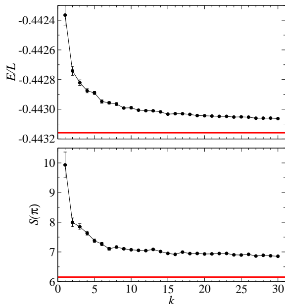
FIG. 20: (Color online) Convergence of the energy per spin (top panel) and the staggered spin structure factor (bottom panel) as a function of the iteration number k for a 1D Heisenberg chain with L = 256 sites and all correlation amplitudes (i.e., r_{\max} = L/2 - 1 ) included in the CAP wave function (7). For each k , 100 adjustments of the parameters were carried out, each based on an MC simulation with 10^4 k^2 updating sweeps. The points with error bars correspond to averages over the last 20 iterations for each k . The horizontal lines are results of unbiased QMC calculations. 56
