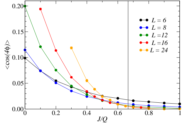
FIG. 17: (Color online) The degree of Z_4 anisotropy of the VBS order parameter of the J - Q model with 6-spin interactions for different system sizes. Here the curve crossings tending to \langle \cos(4\phi) \rangle = 0 with increasing L demonstrates the emergent U(1) symmetry at the Néel-VBS transition of this model.
