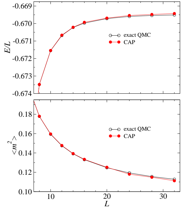
FIG. 25: (Color online) Energy (top panel) and squared sublattice magnetization (bottom panel) of the 2D Heisenberg model obtained by unbiased QMC calculations and by optimized CAP state with all bond correlations included. 56
